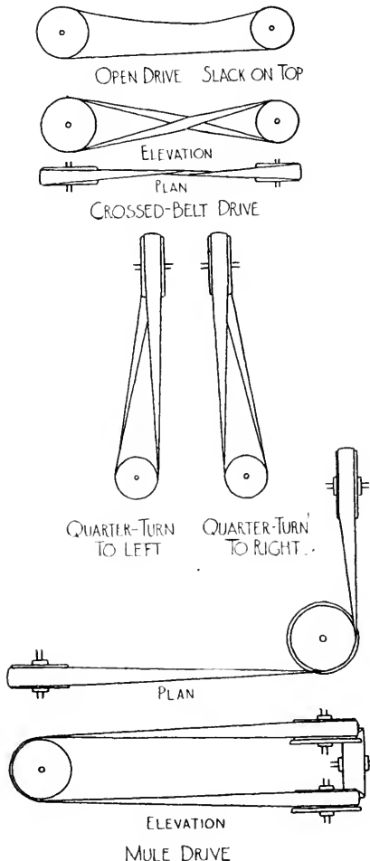
FIG. 230. COMMON "DRIVES."
